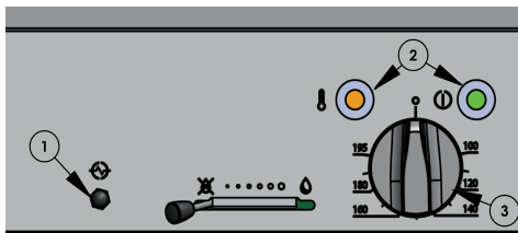
Figure 10 Device controls
