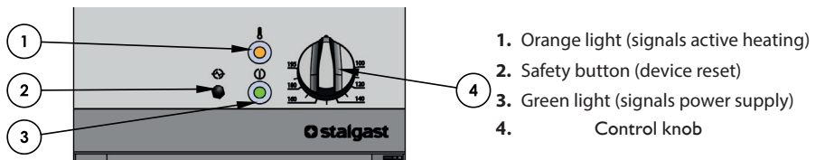
Figure 8 Device controls
